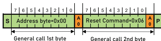
Figure 19: Reset through general call
